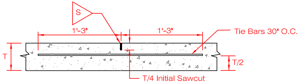
(E) LONGITUDINAL CONTRACTION JOINT
