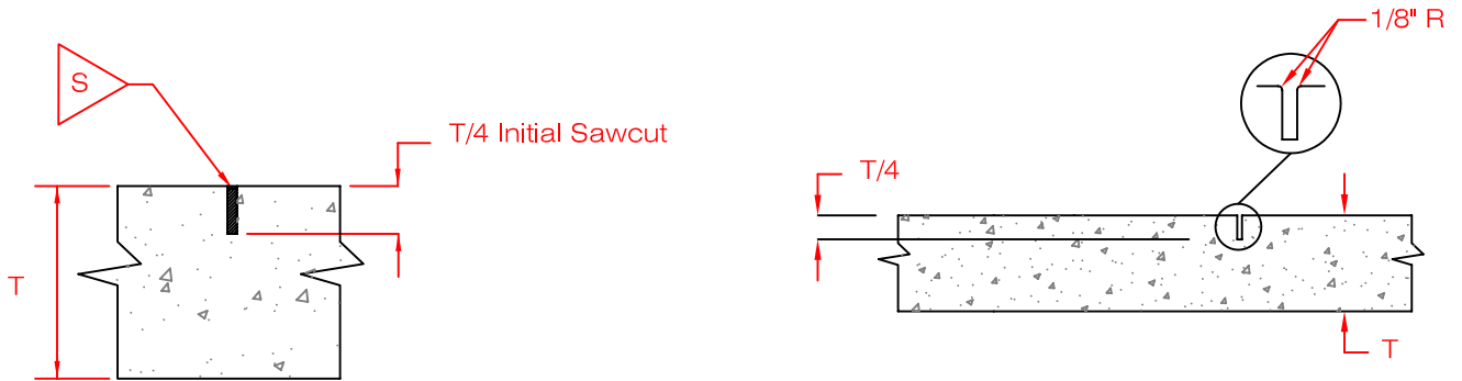
(C) TRANSVERSE CONTRACTION JOINT (T) TOOLED CONTRACTION JOINT
