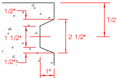
KEYWAY DETAIL
