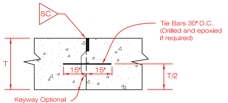
(L) CONSTRUCTION JOINT
