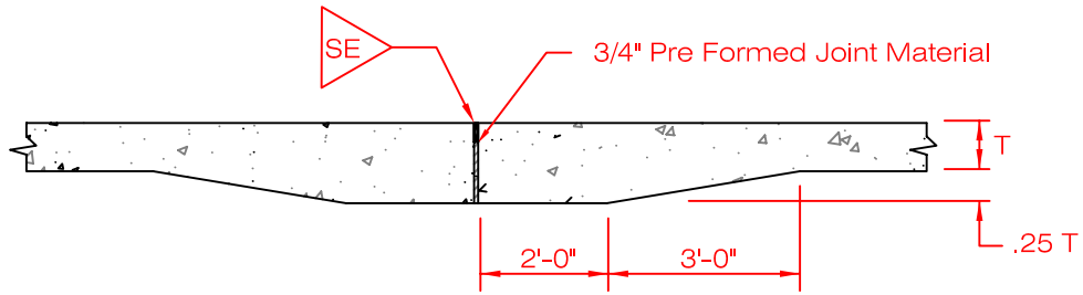
(A) EXPANSION JOINT (THICKENED EDGE)
