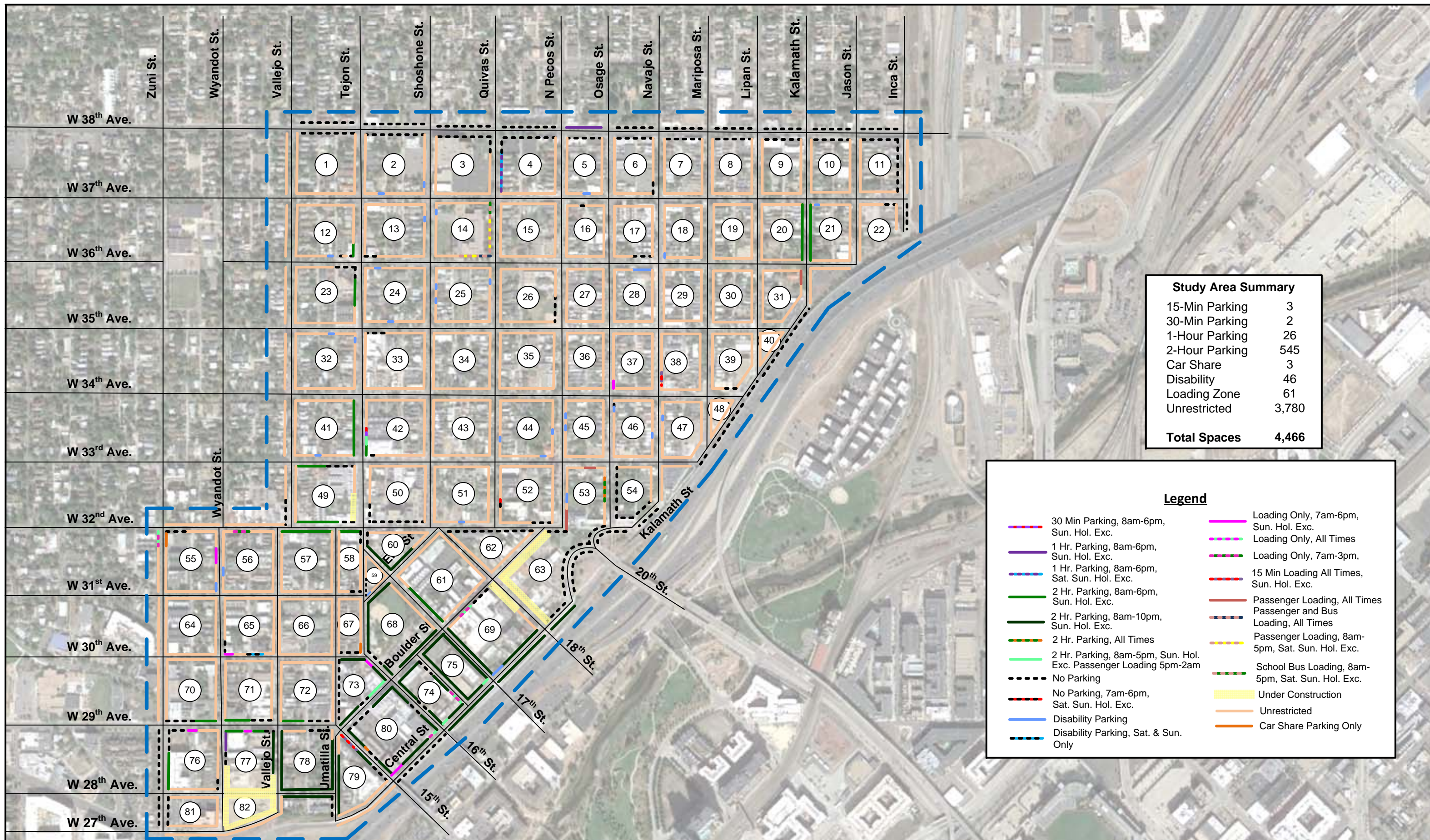
Figure 1 Lower Highlands Parking Restrictions
