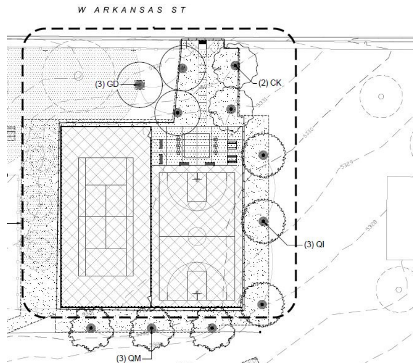
Technical layout of the new tennis court and basketball court
