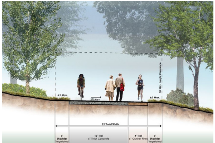
Denver Parks and Recreation's Regional Trail Cross-Section
